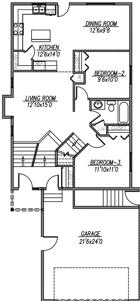
MAIN FLOOR 1053 SQ. FT.
