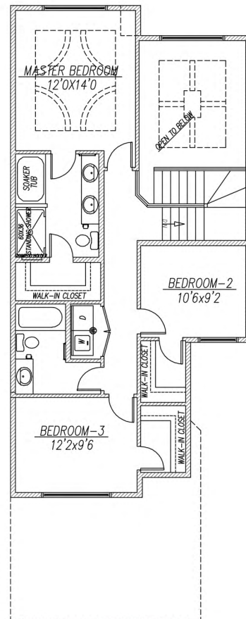
UPPER FLOOR 825 SQ. FT.
