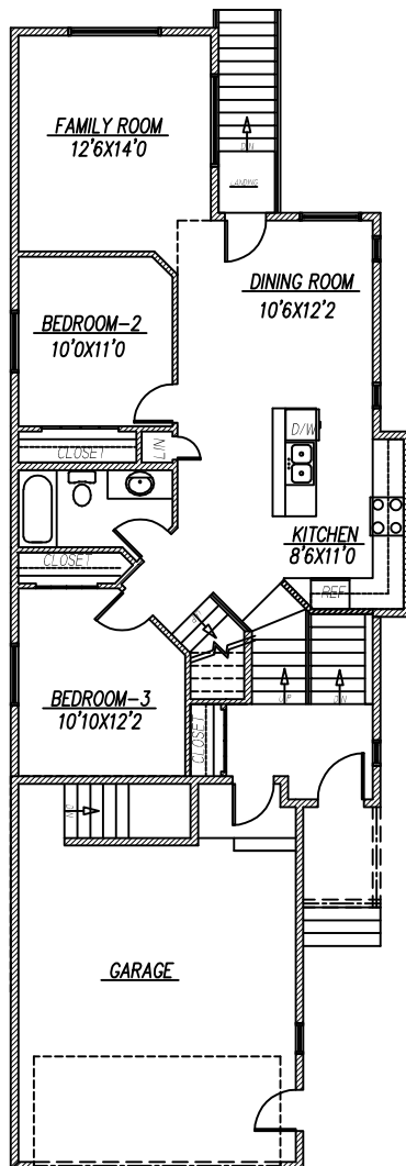
MAIN FLOOR 1084 SQ. FT.
