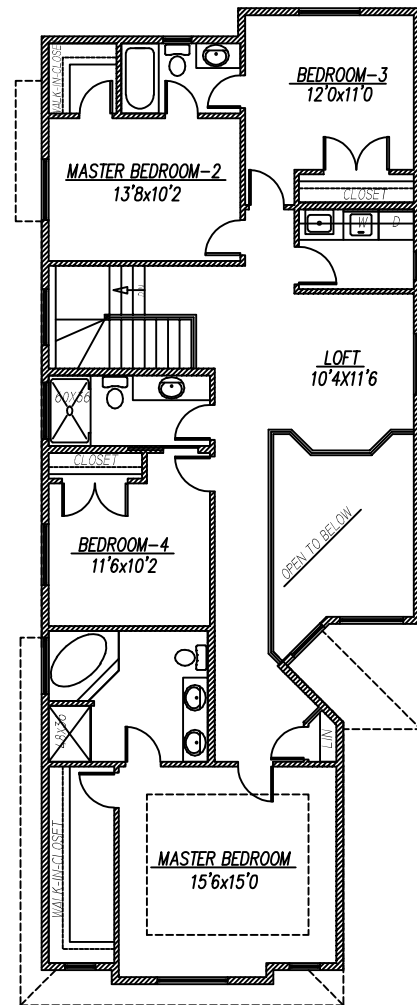
UPPER FLOOR 1476 SQ. FT.
