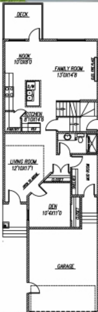
MAIN FLOOR 1064 SQ. FT.
